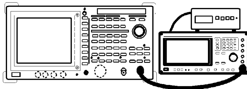
Figure 1-2 Connections for Measuring the Frequency Reference Output Accuracy (when the OPT21, OPT22 and OPT23 are installed)
