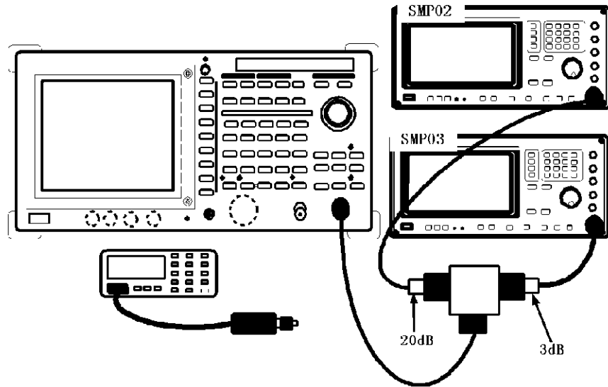
Figure 1-11 Setup for the Gain Compression
